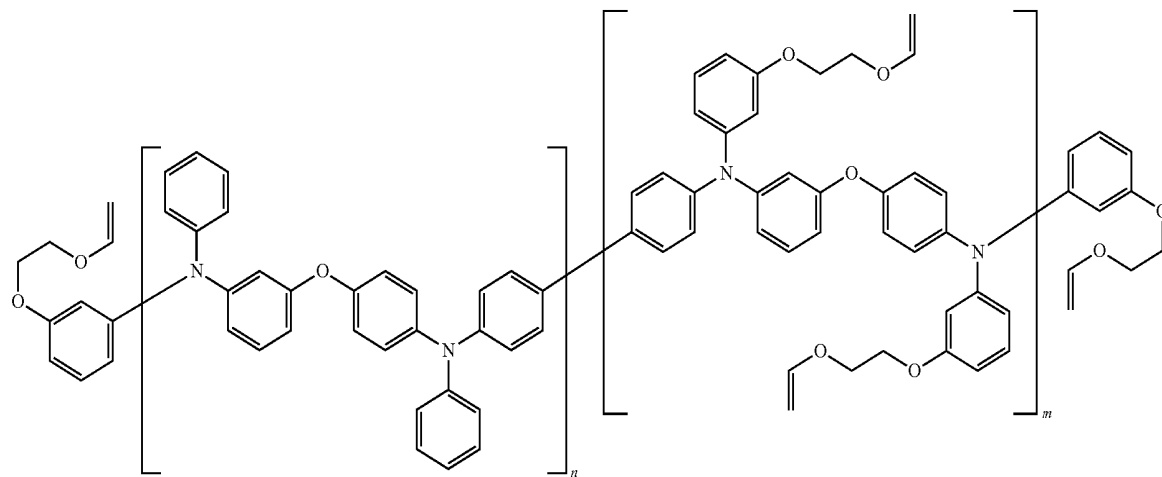
[Formula 34]
