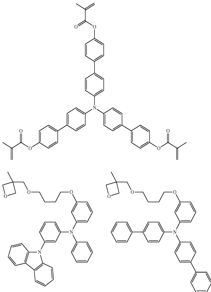
[Formula 31]
