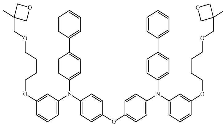
[Formula 29]
