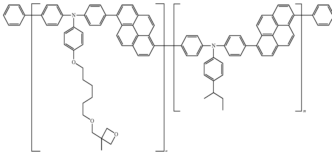
[Formula 39]
