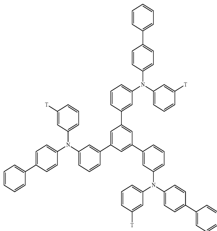
[Formula 21]
