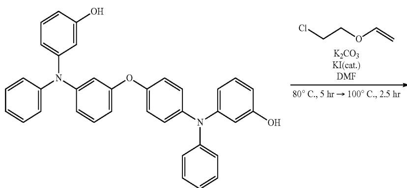
Target compound 26
