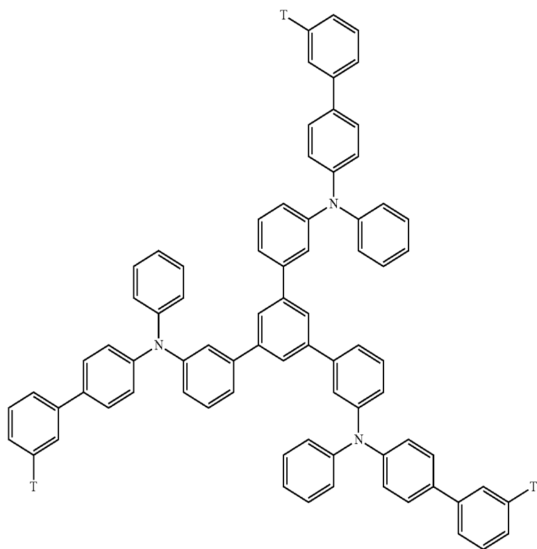
[Formula 14]
