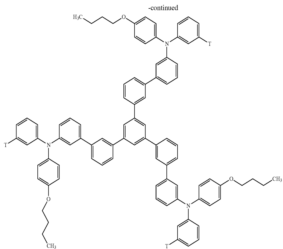
[Formula 21]
