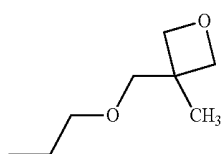
[Formula 7]
