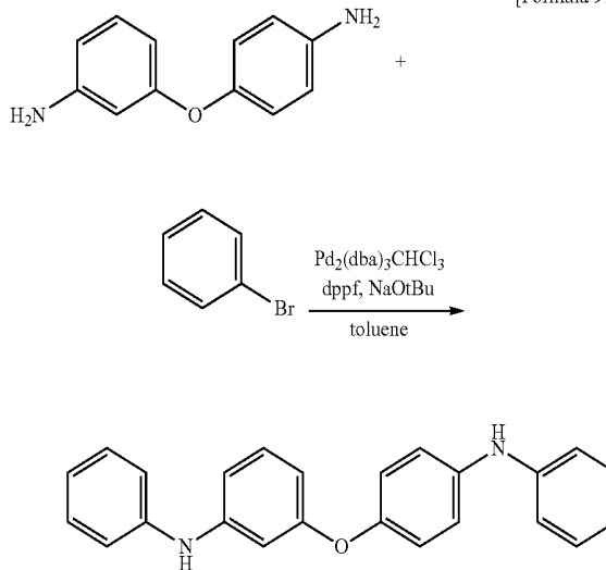
(Target compound 24)
