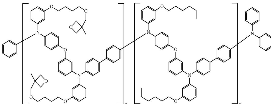
[Formula 31]
