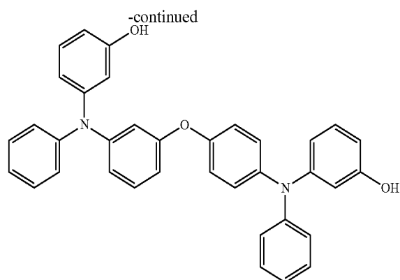
Target compound 26
