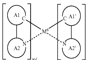
[Formula 61]
