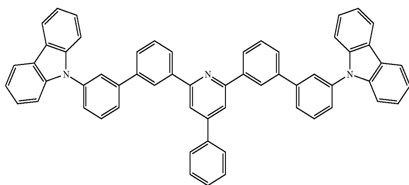
[Formula 66]
