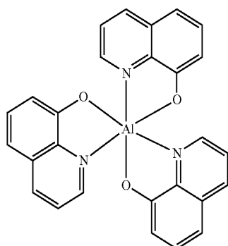
[Formula 102]
