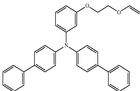
(Target compound 23)
