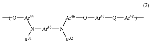
[Formula 44]
