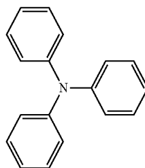
[Formula 9]
