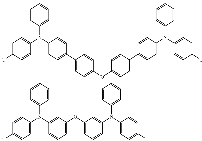
[Formula 24]
