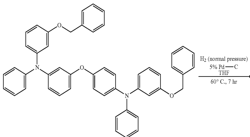
Target compound 25
