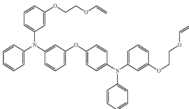
Target compound 27
