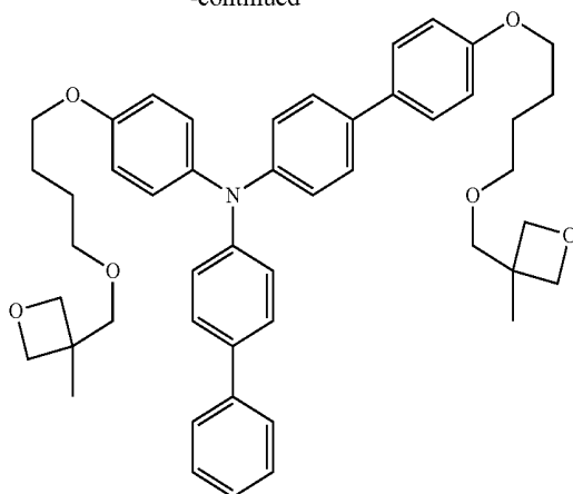
Target compound 8
