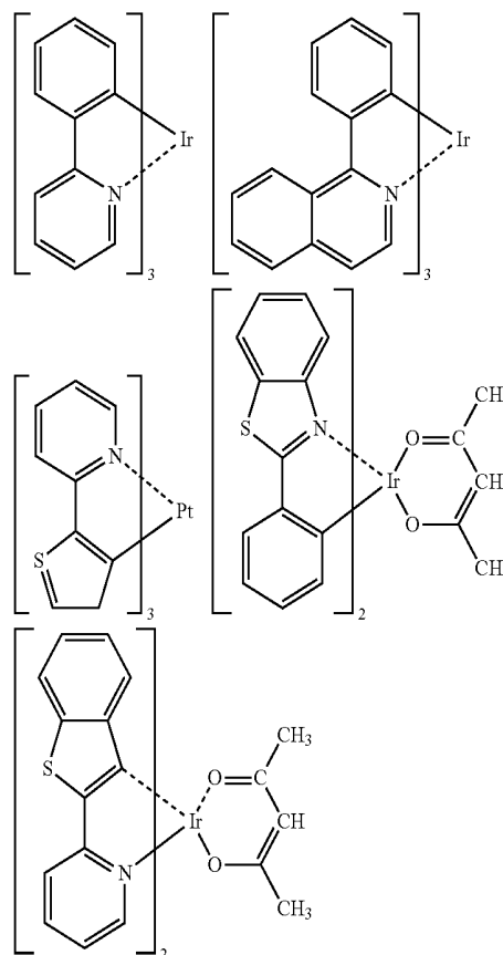
[Formula 62]
